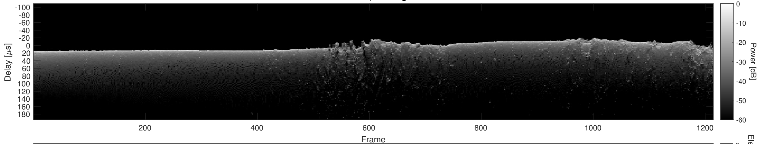
Orbit 13611, Cluttergram
