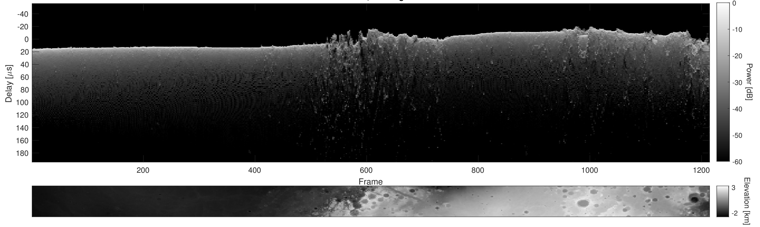
Orbit 13611, Cluttergram
