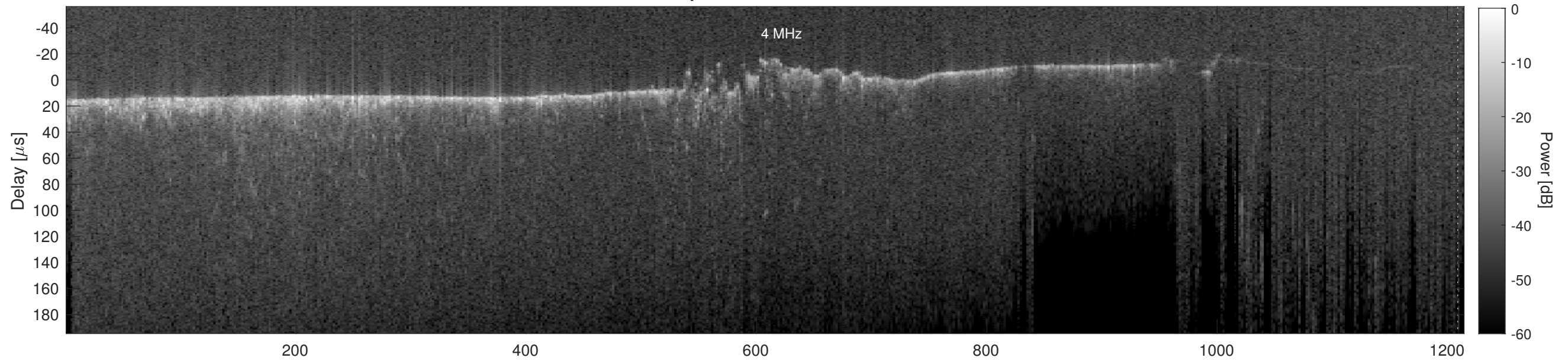
Orbit 13611, Cluttergram
