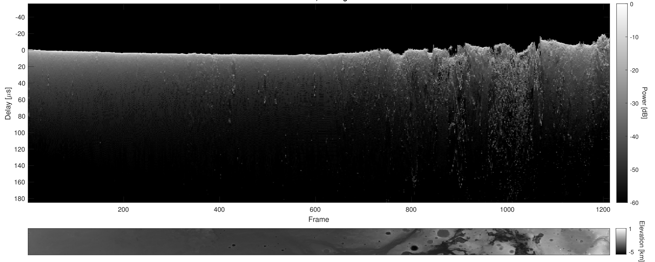
Orbit 13612, Cluttergram
