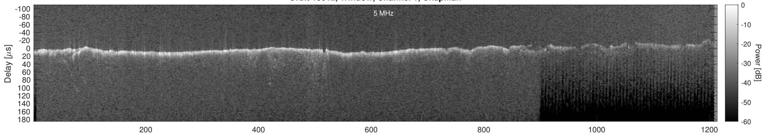
Orbit 13612, Window, Channel 1, Optimized
