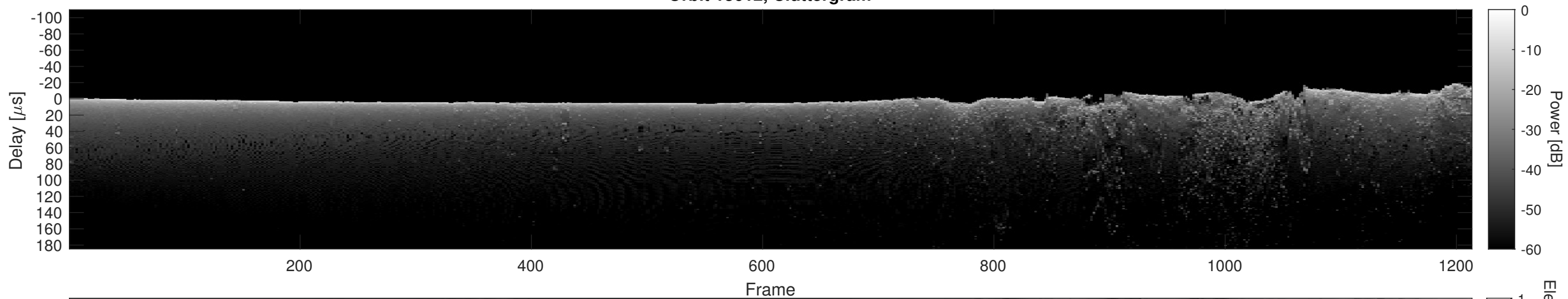
Orbit 13612, Cluttergram
