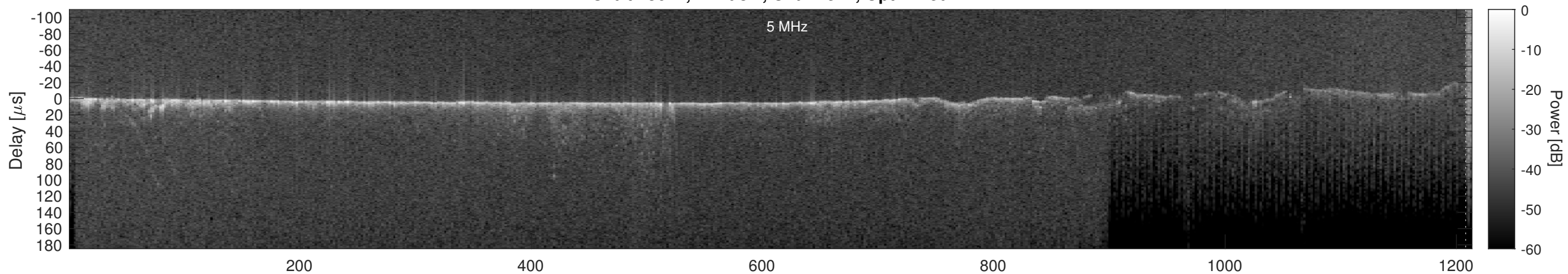
Orbit 13612, Cluttergram
