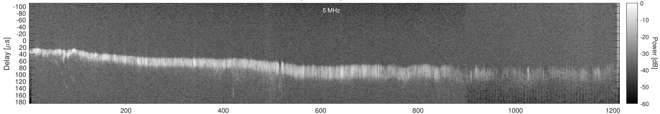
Orbit 13612, Window, Channel 1, Chapman
