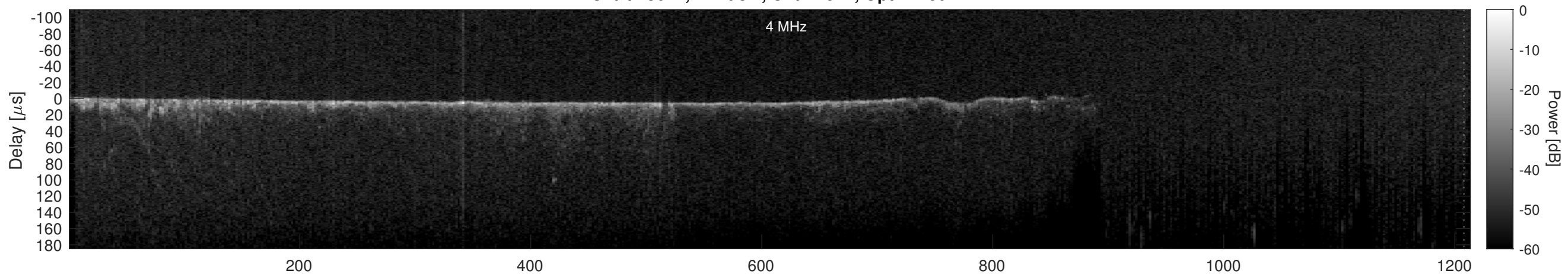
Orbit 13612, Cluttergram
