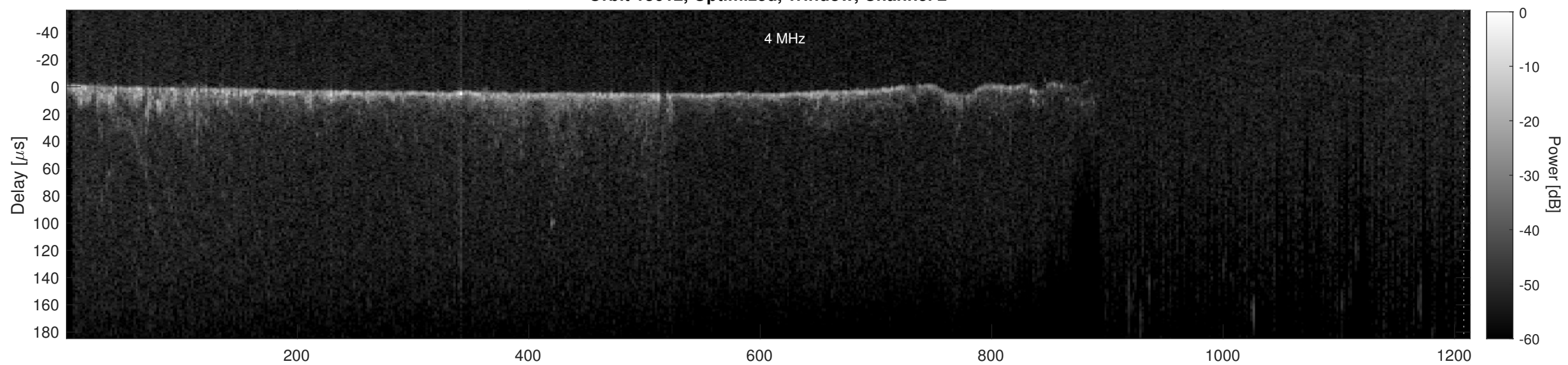
Orbit 13612, Cluttergram
