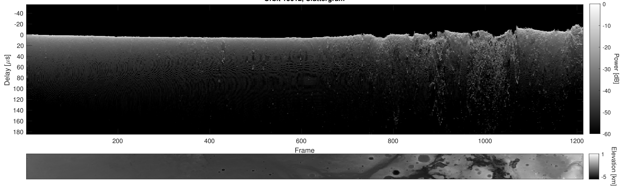
Orbit 13612, Cluttergram
