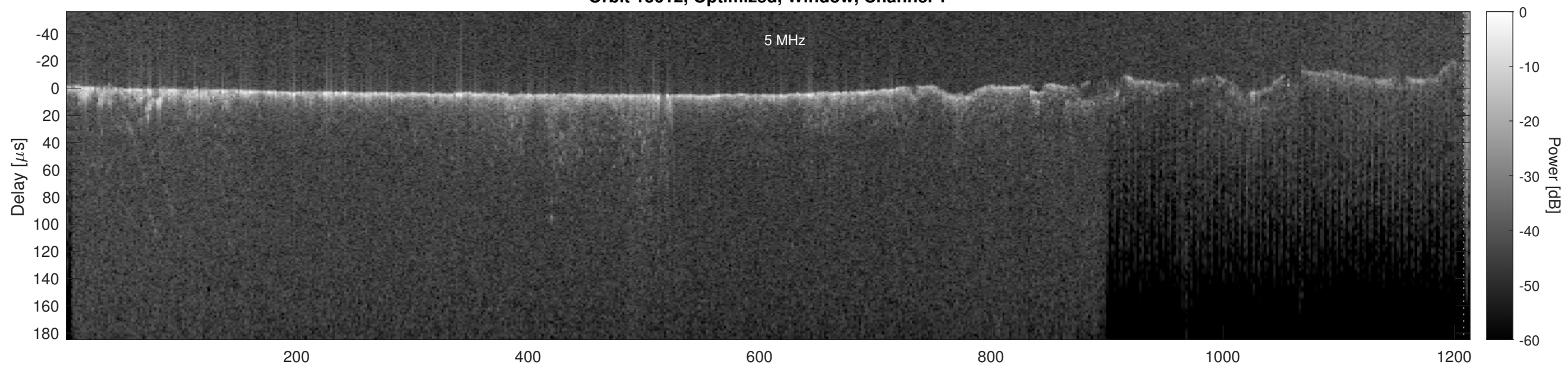
Orbit 13612, Optimized, Window, Channel 2
