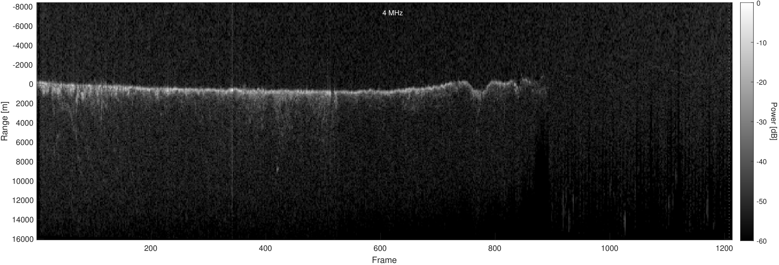
Orbit 13612, Optimized, Window, Depth-Corrected, Channel 2
