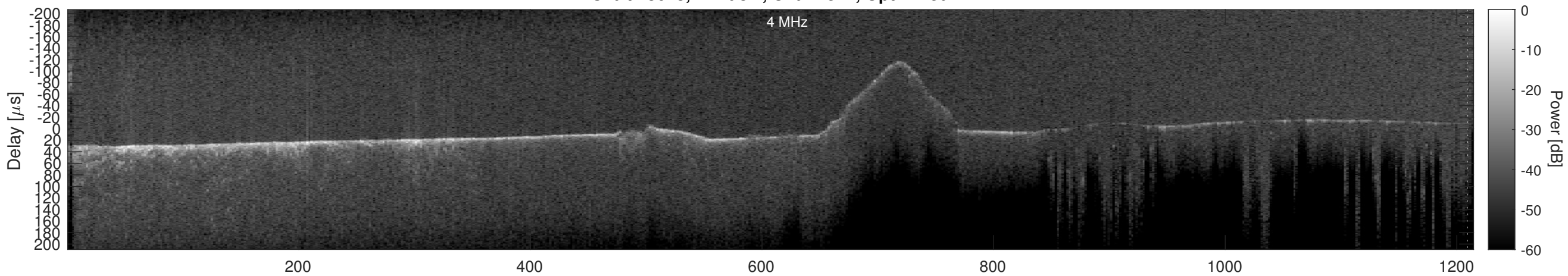
Orbit 13613, Cluttergram
