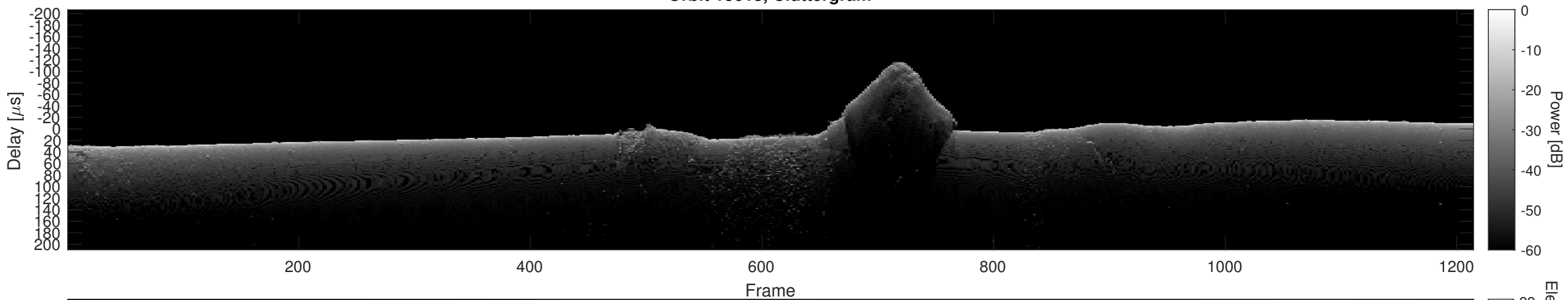
Orbit 13613, Cluttergram
