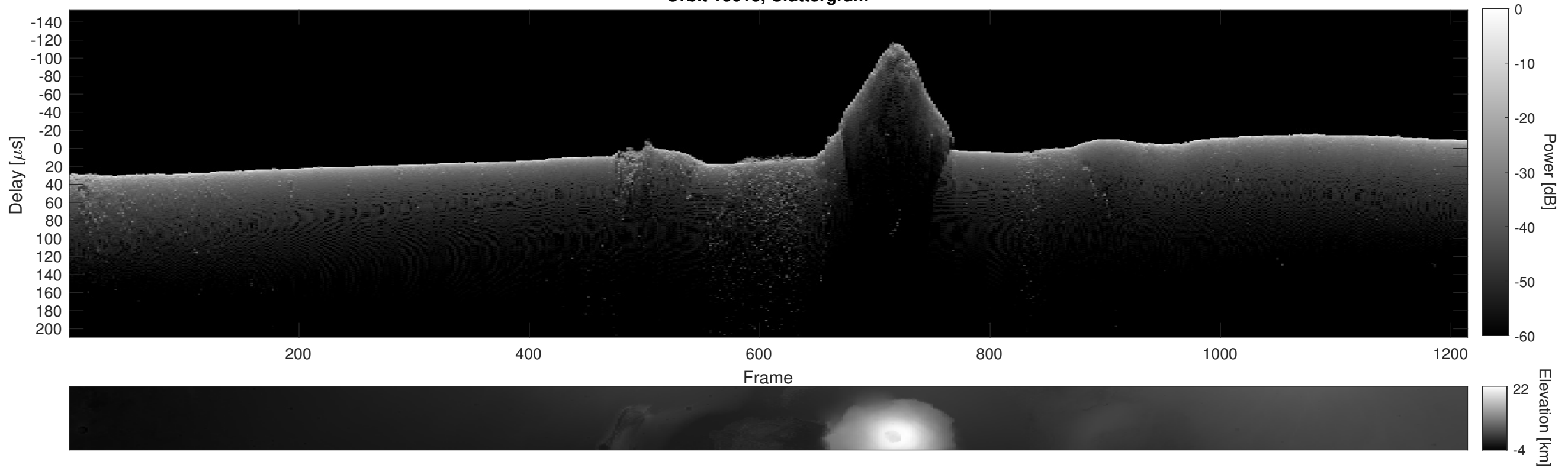
Orbit 13613, Cluttergram
