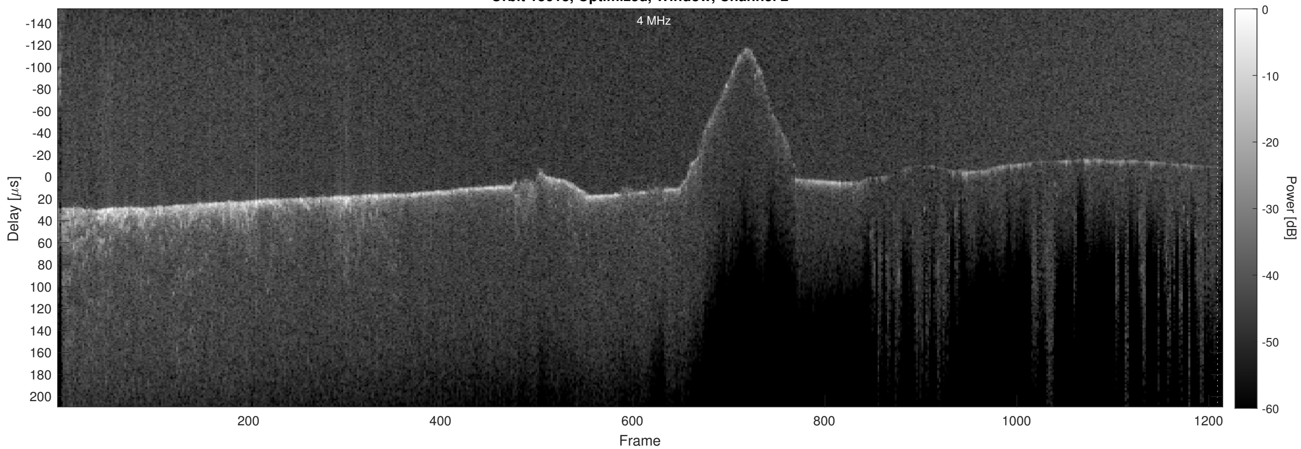
Orbit 13613, Optimized, Window, Channel 2
