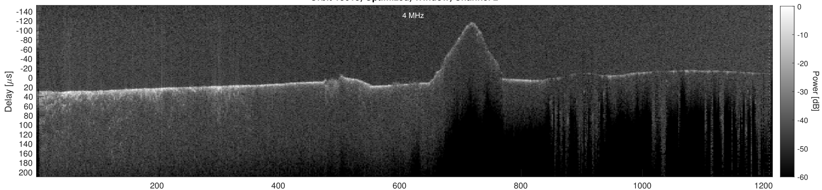
Orbit 13613, Cluttergram
