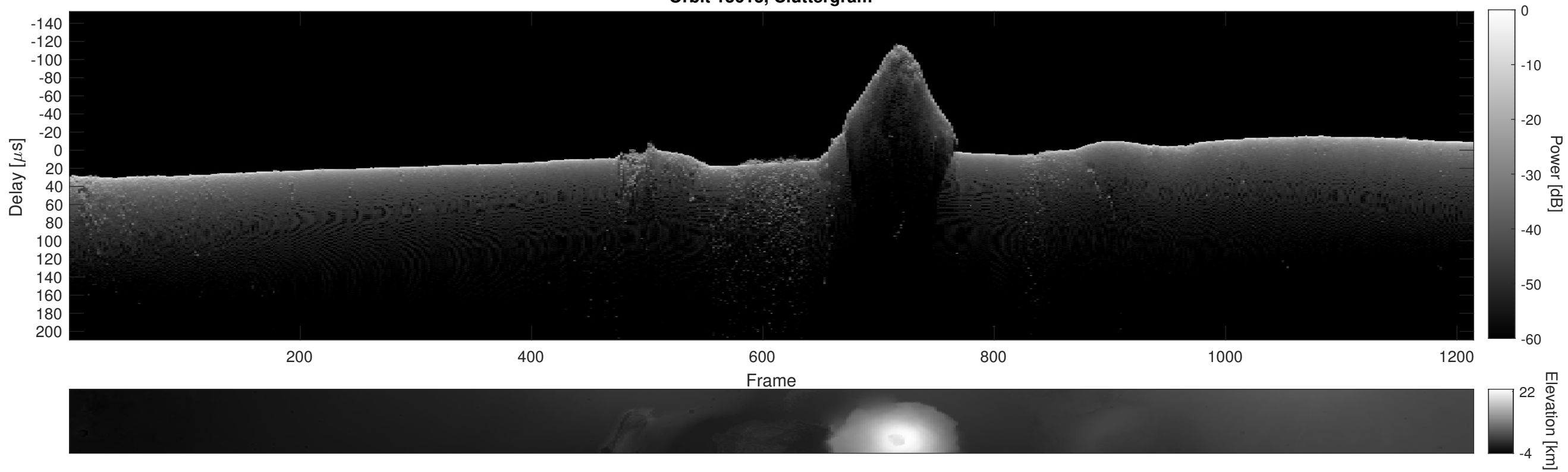
Orbit 13613, Cluttergram
