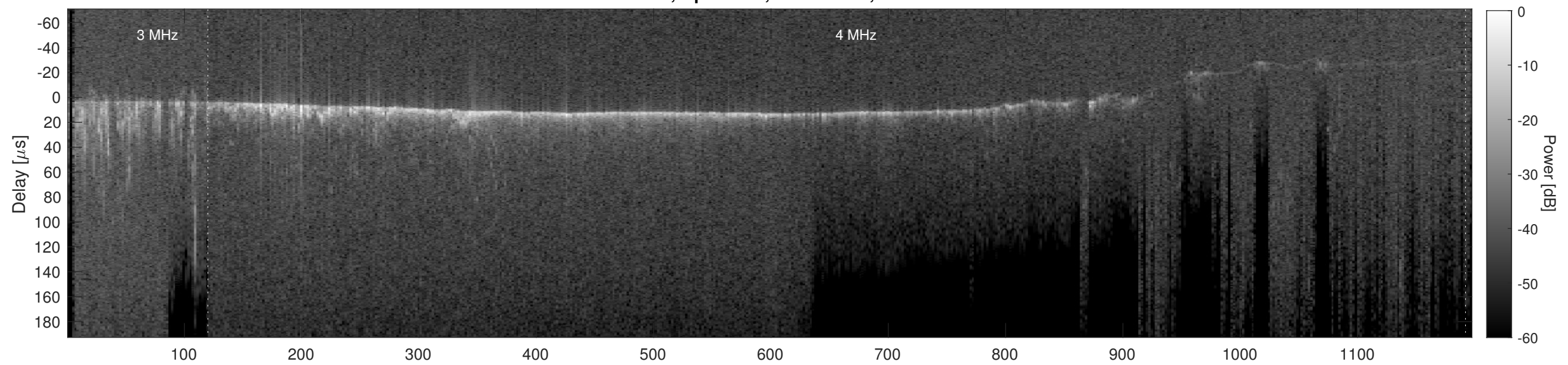
Orbit 13614, Cluttergram
