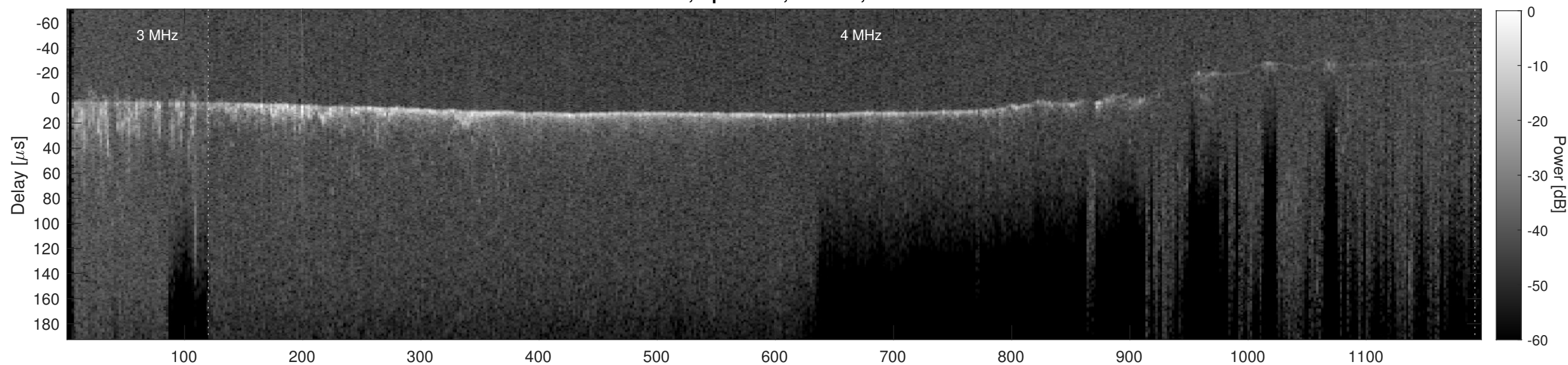
Orbit 13614, Cluttergram
