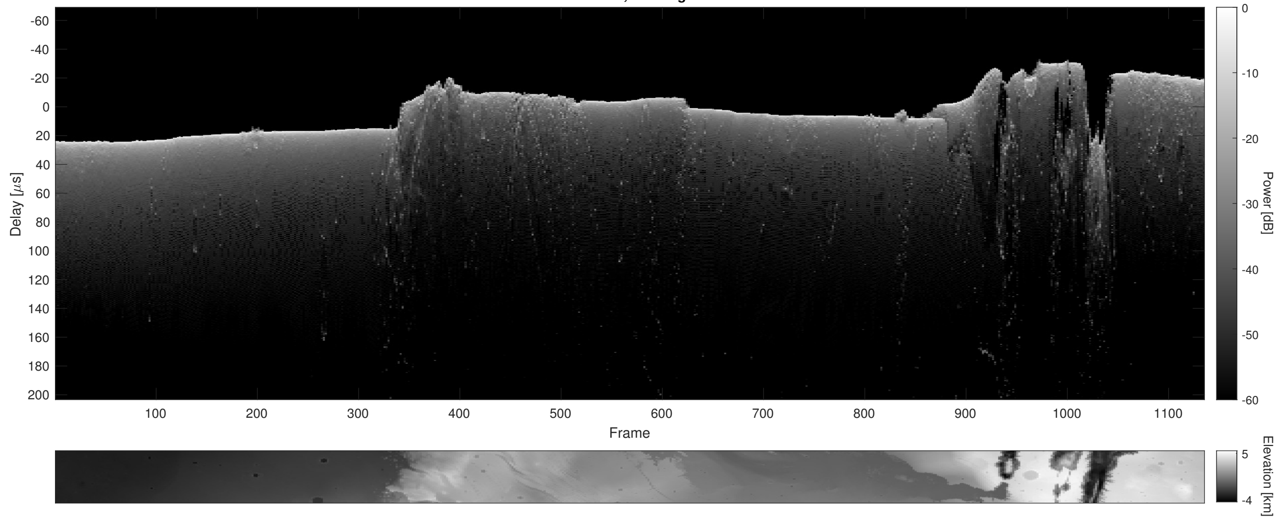
Orbit 13616, Cluttergram
