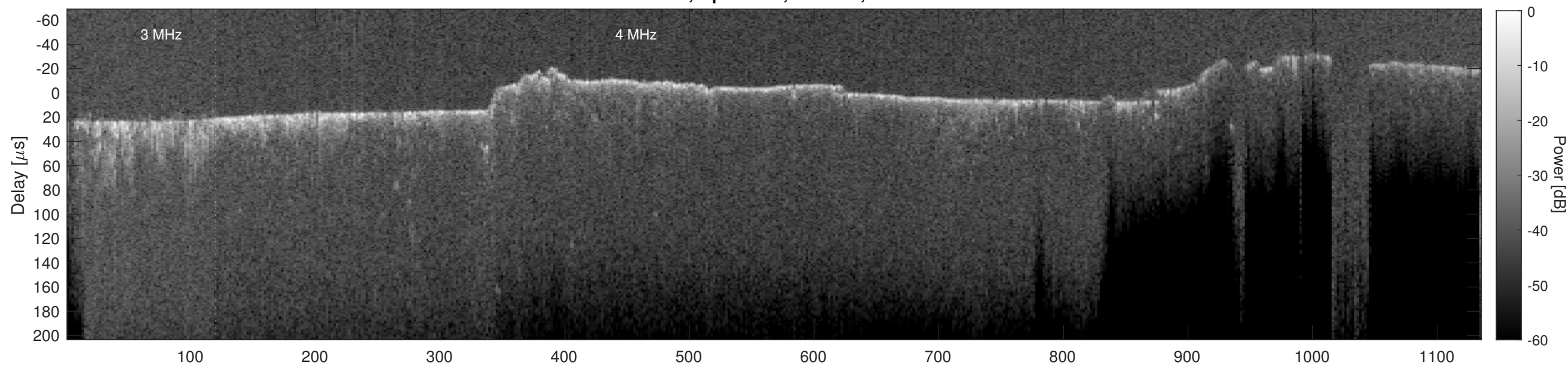
Orbit 13616, Cluttergram
