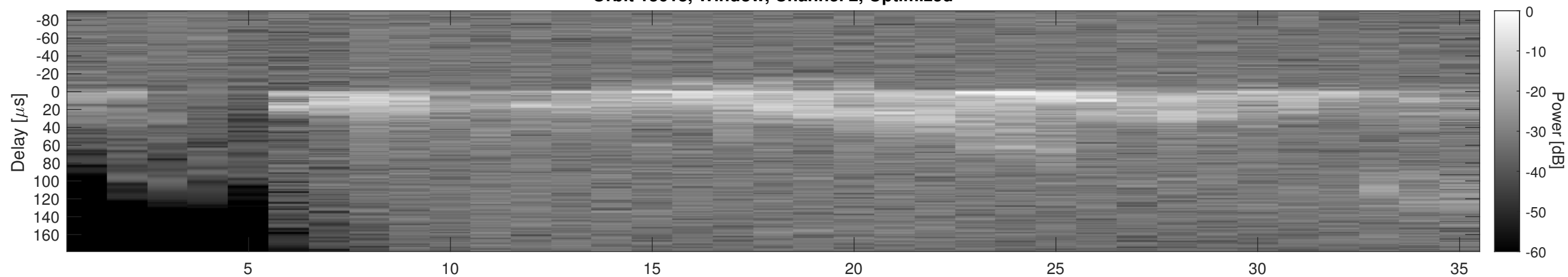
Orbit 13618, Cluttergram
