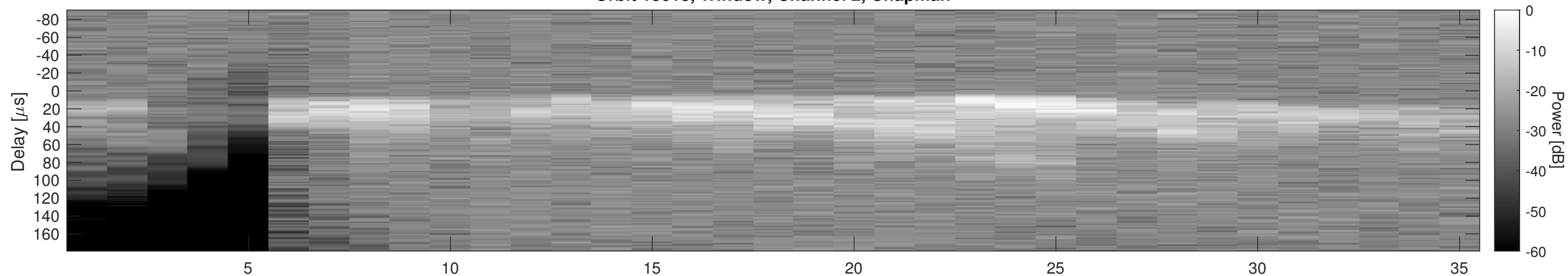
Orbit 13618, Window, Channel 2, Optimized
