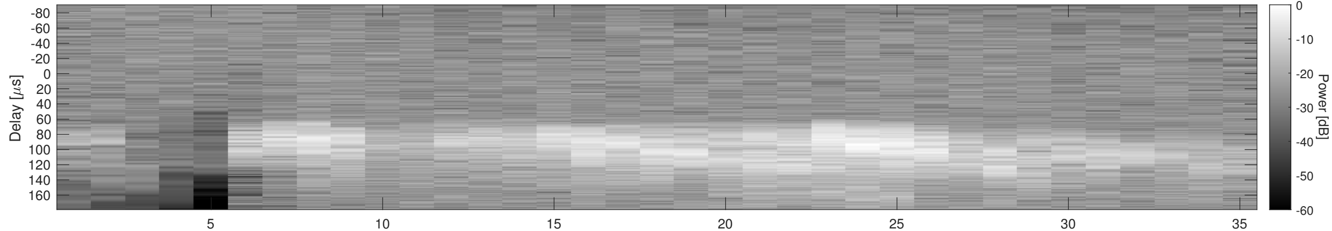
Orbit 13618, Window, Channel 2, Chapman
