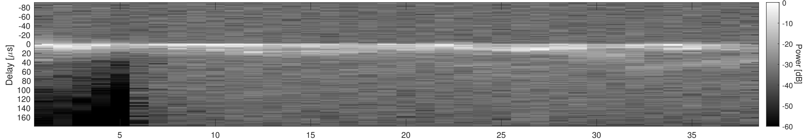
Orbit 13619, Cluttergram
