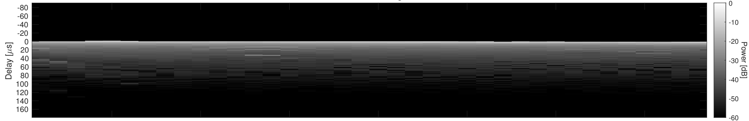
Orbit 13619, Cluttergram
