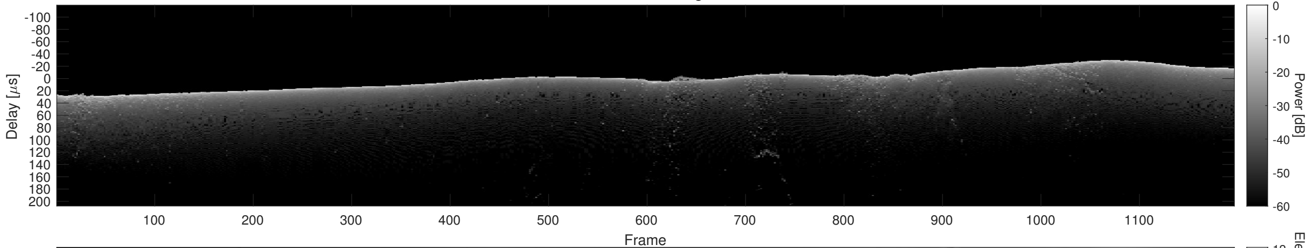
Orbit 13620, Cluttergram
