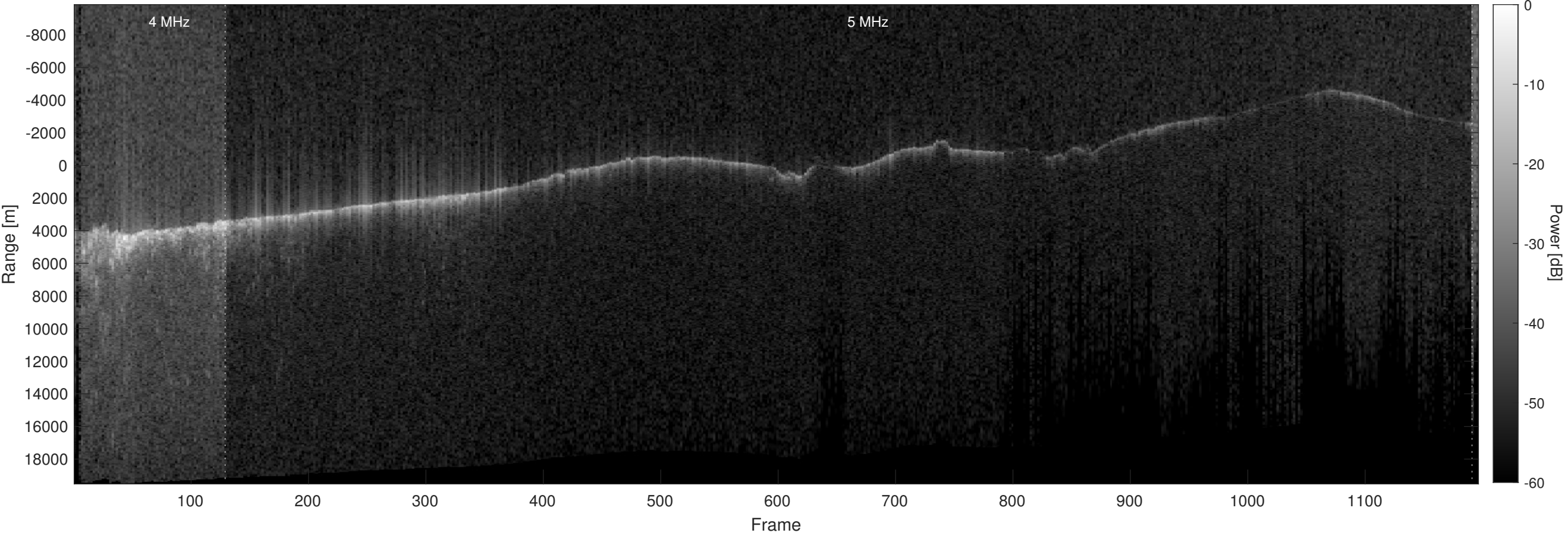
Orbit 13620, Optimized, No Window, Depth-Corrected, Channel 2
