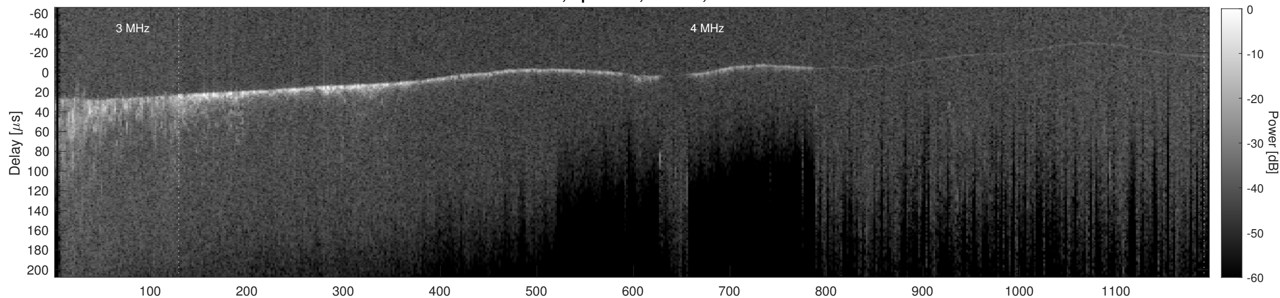
Orbit 13620, Cluttergram
