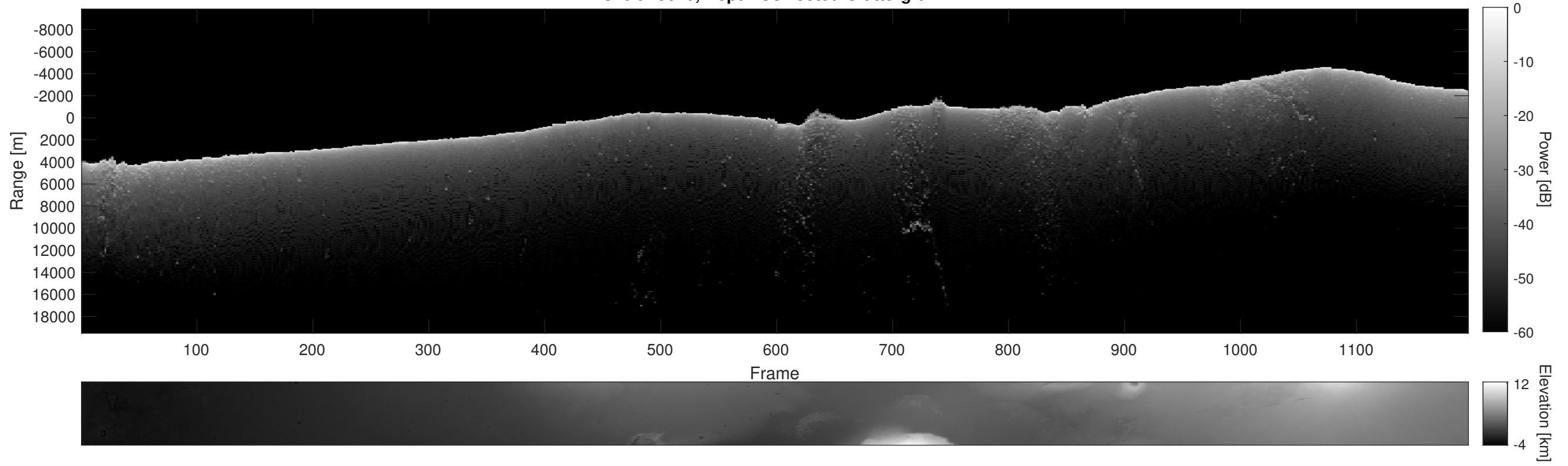
Orbit 13620, Depth-Corrected Cluttergram
