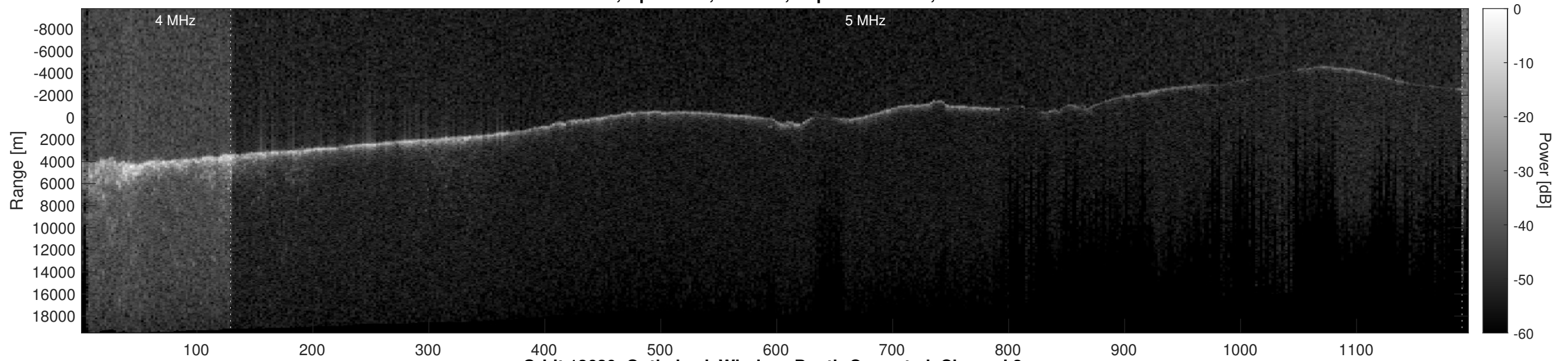
Orbit 13620, Optimized, Window, Depth-Corrected, Channel 2
