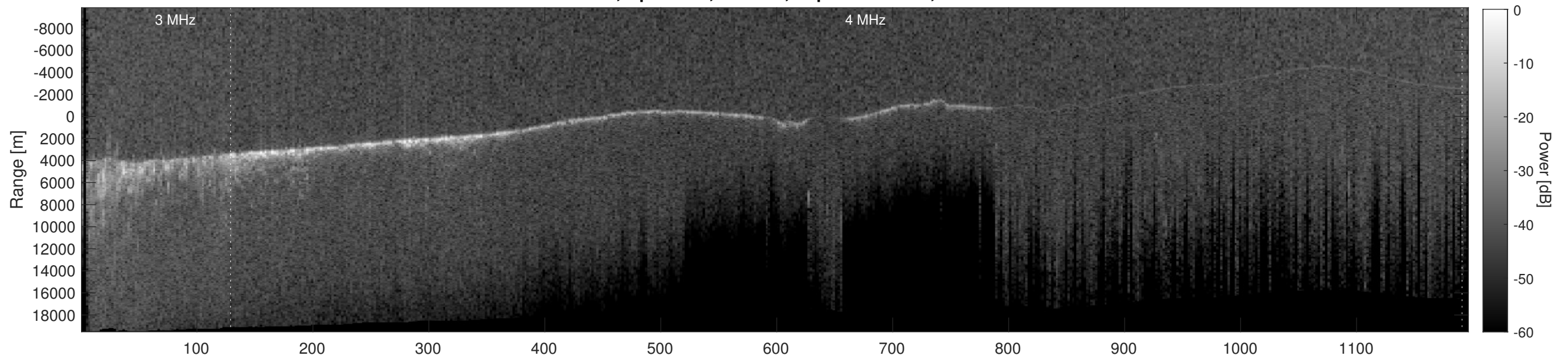
Orbit 13620, Depth-Corrected Cluttergram
