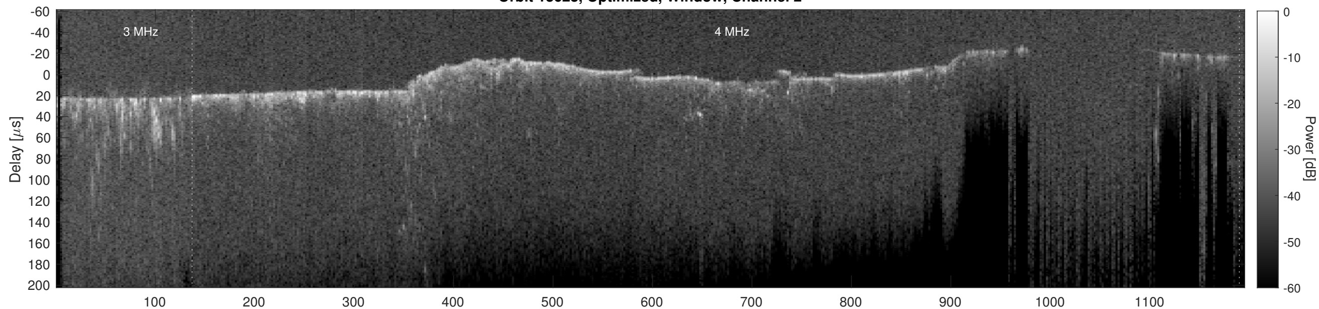
Orbit 13623, Cluttergram
