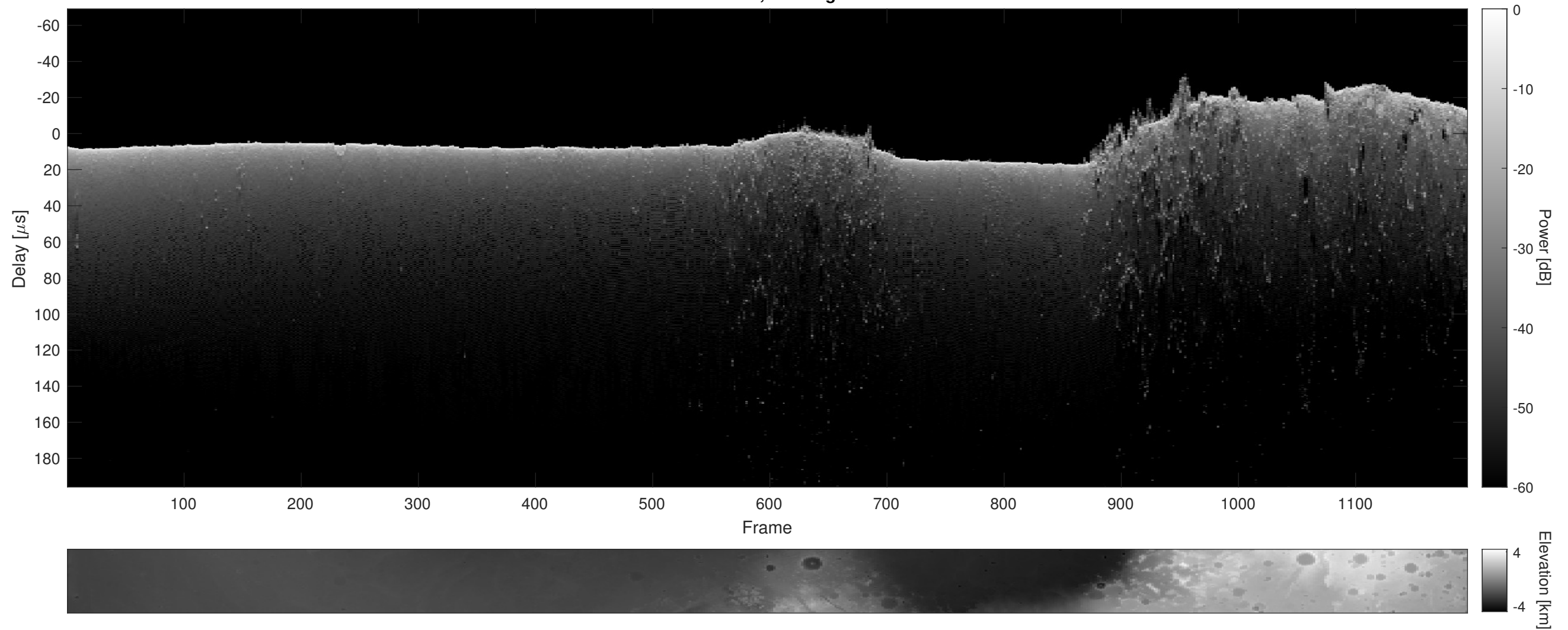
Orbit 13625, Cluttergram
