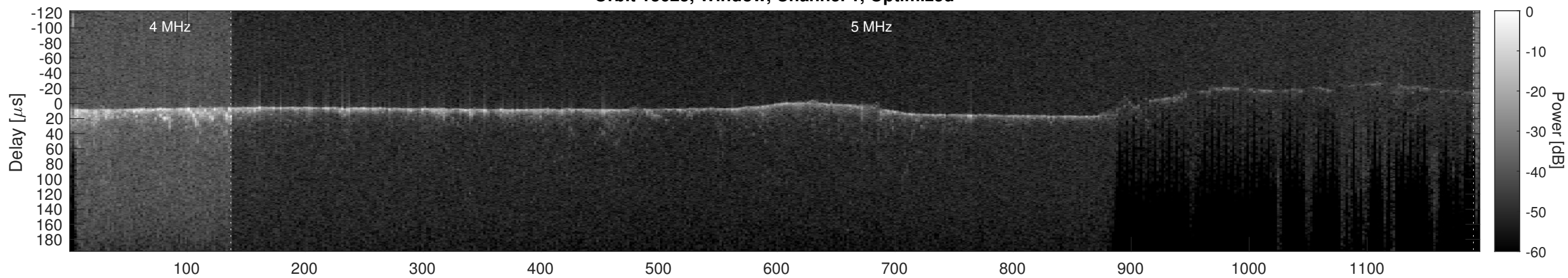
Orbit 13625, Cluttergram
