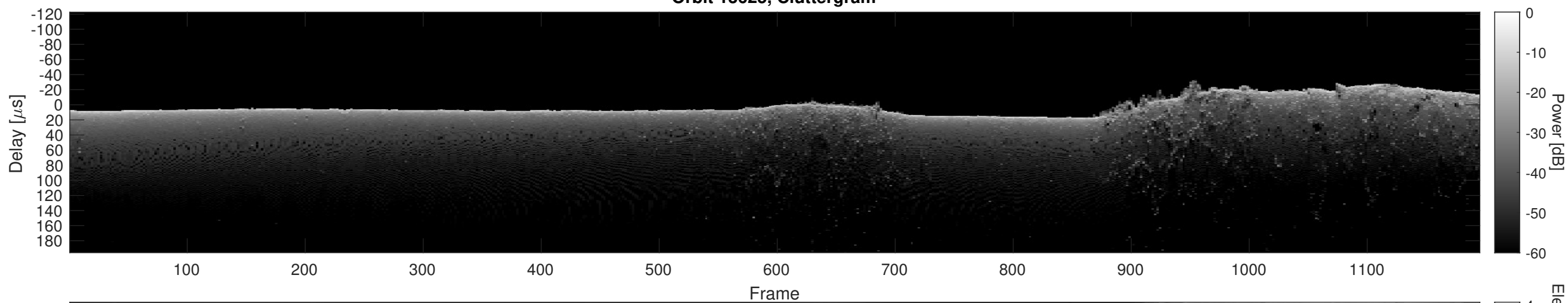
Orbit 13625, Cluttergram
