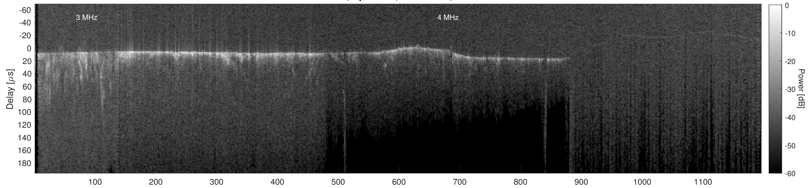
Orbit 13625, Cluttergram
