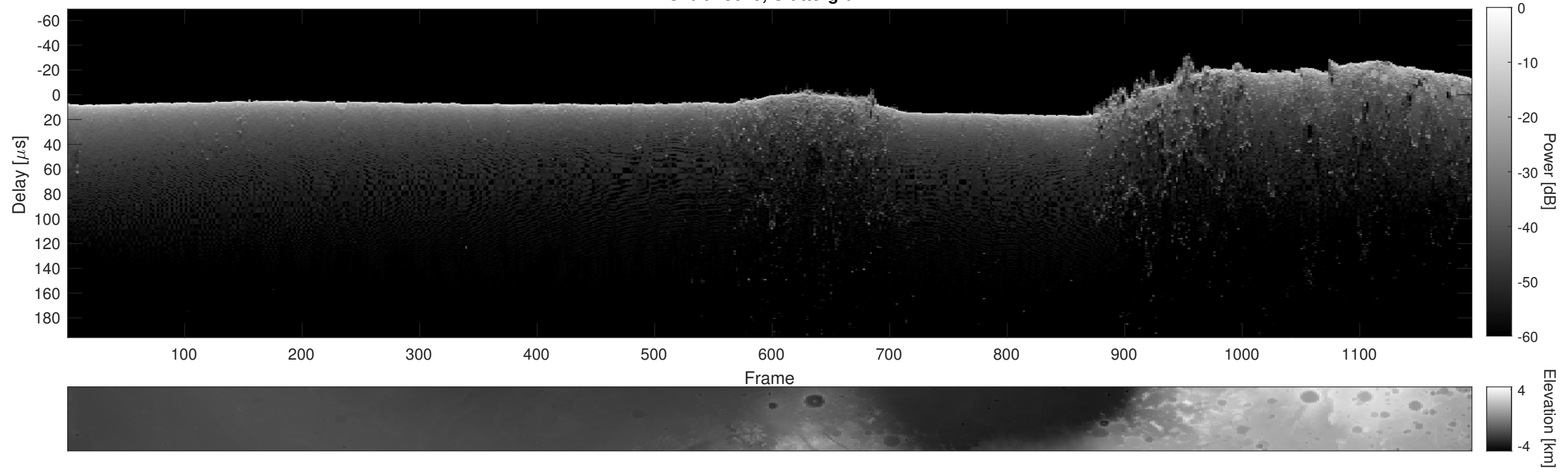
Orbit 13625, Cluttergram
