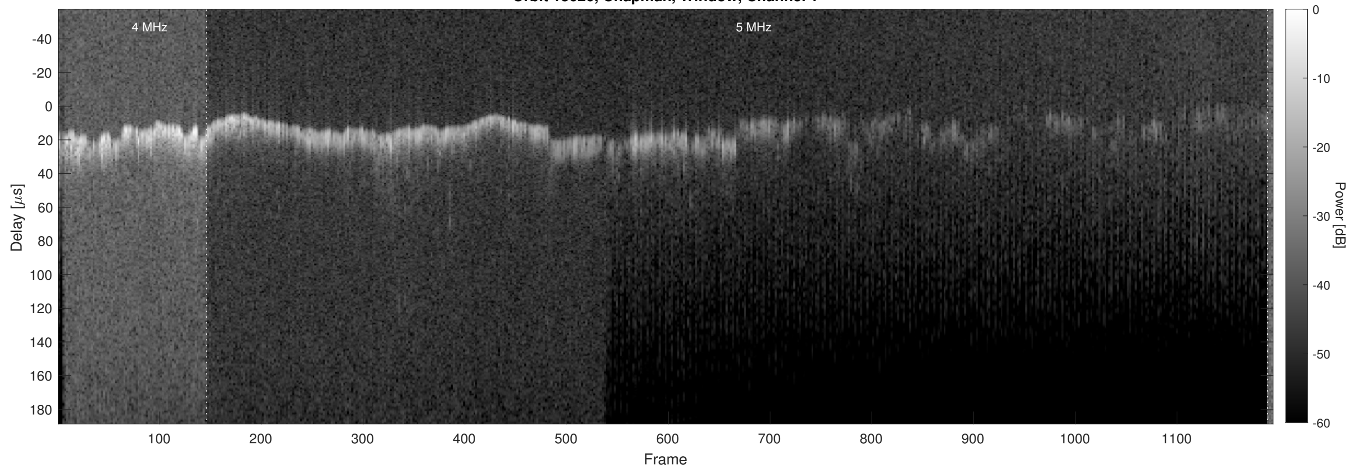
Orbit 13626, Chapman, Window, Channel 2
