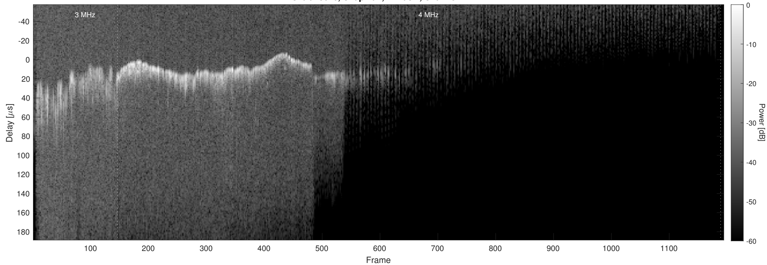
Orbit 13626, Chapman, Window, Channel 2
