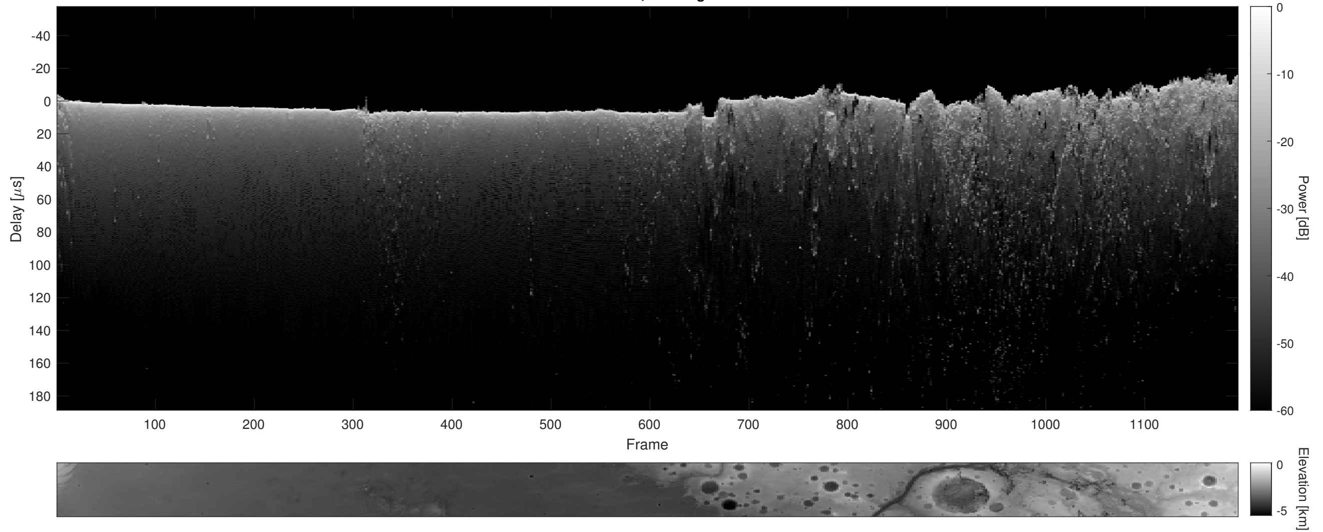
Orbit 13626, Cluttergram
