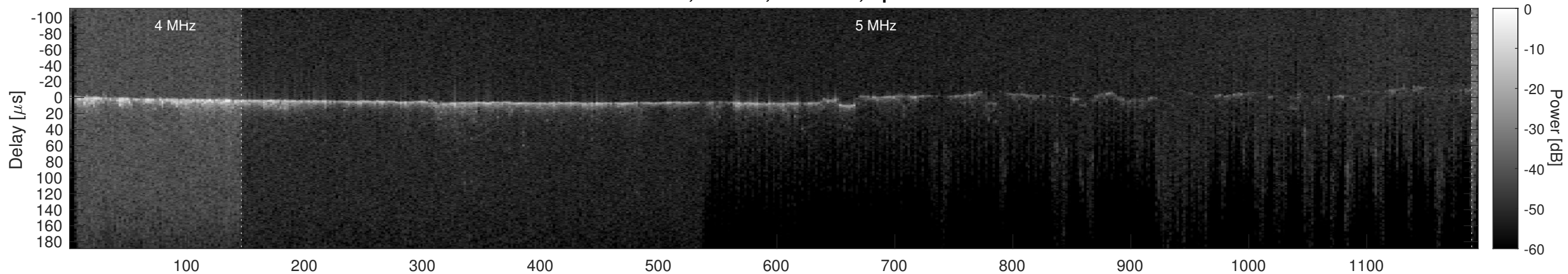
Orbit 13626, Cluttergram
