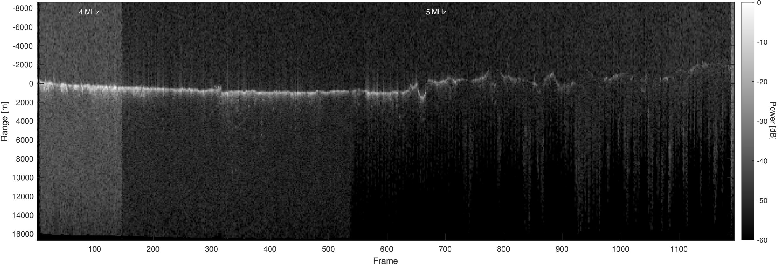
Orbit 13626, Optimized, Window, Depth-Corrected, Channel 2
