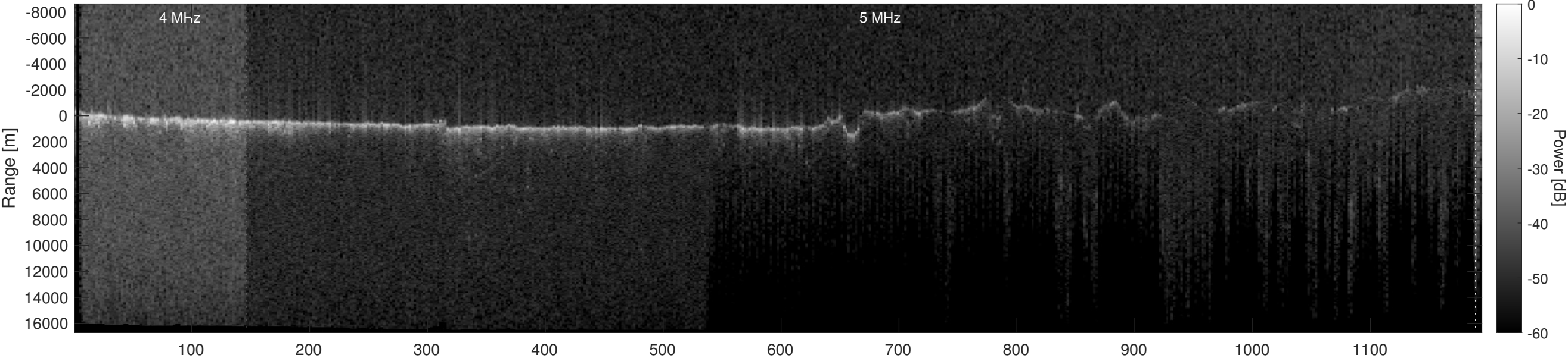
Orbit 13626, Optimized, Window, Depth-Corrected, Channel 2
