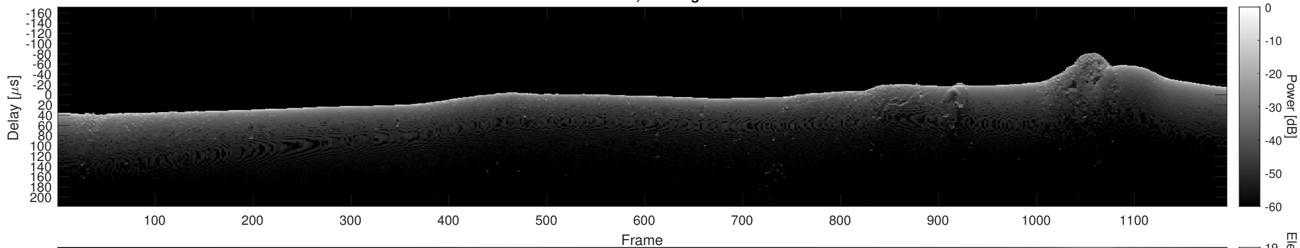
Orbit 13627, Cluttergram
