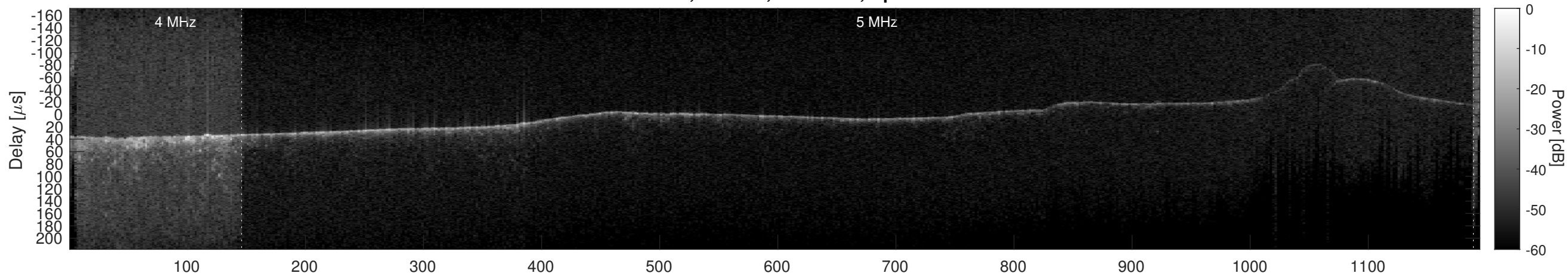
Orbit 13627, Cluttergram
