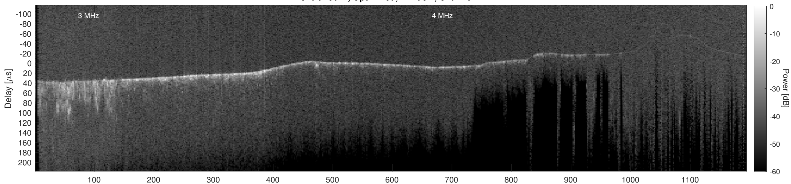
Orbit 13627, Cluttergram
