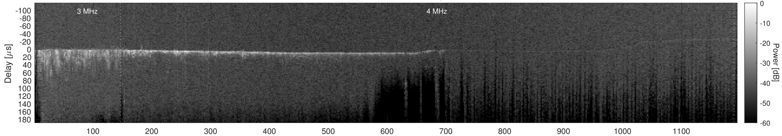
Orbit 13628, Cluttergram
