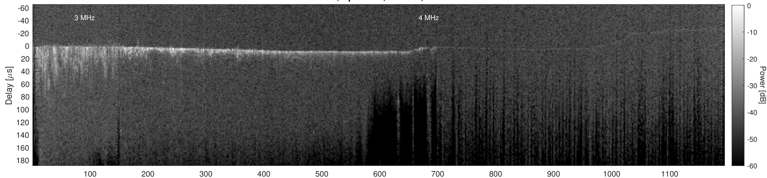
Orbit 13628, Cluttergram
