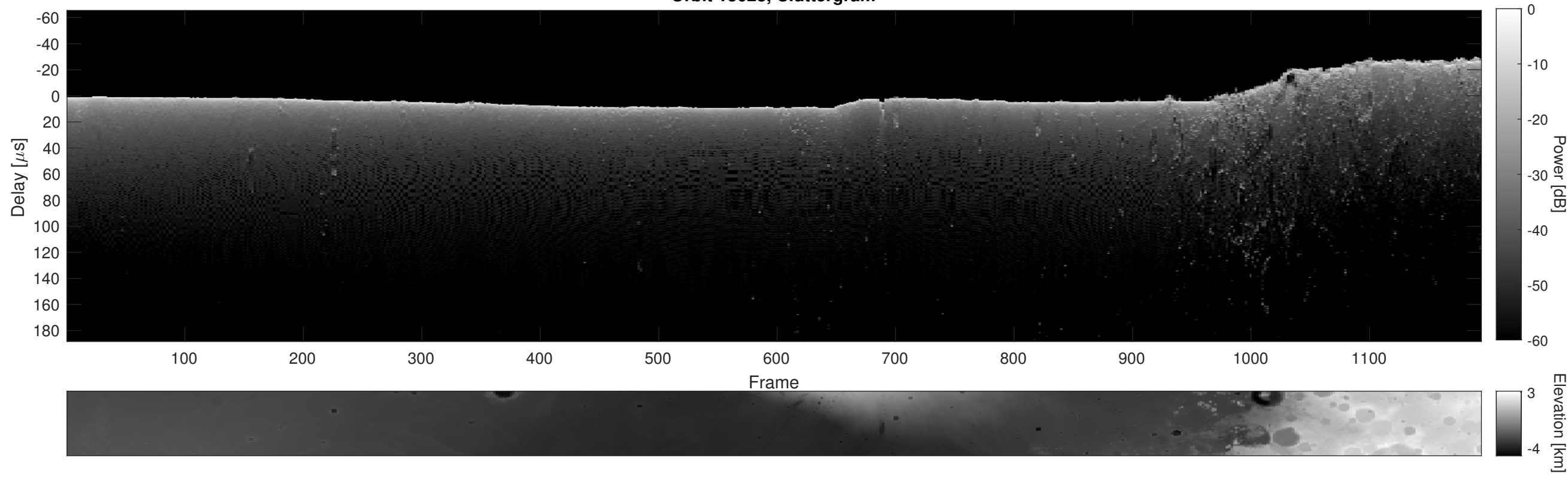
Orbit 13628, Cluttergram
