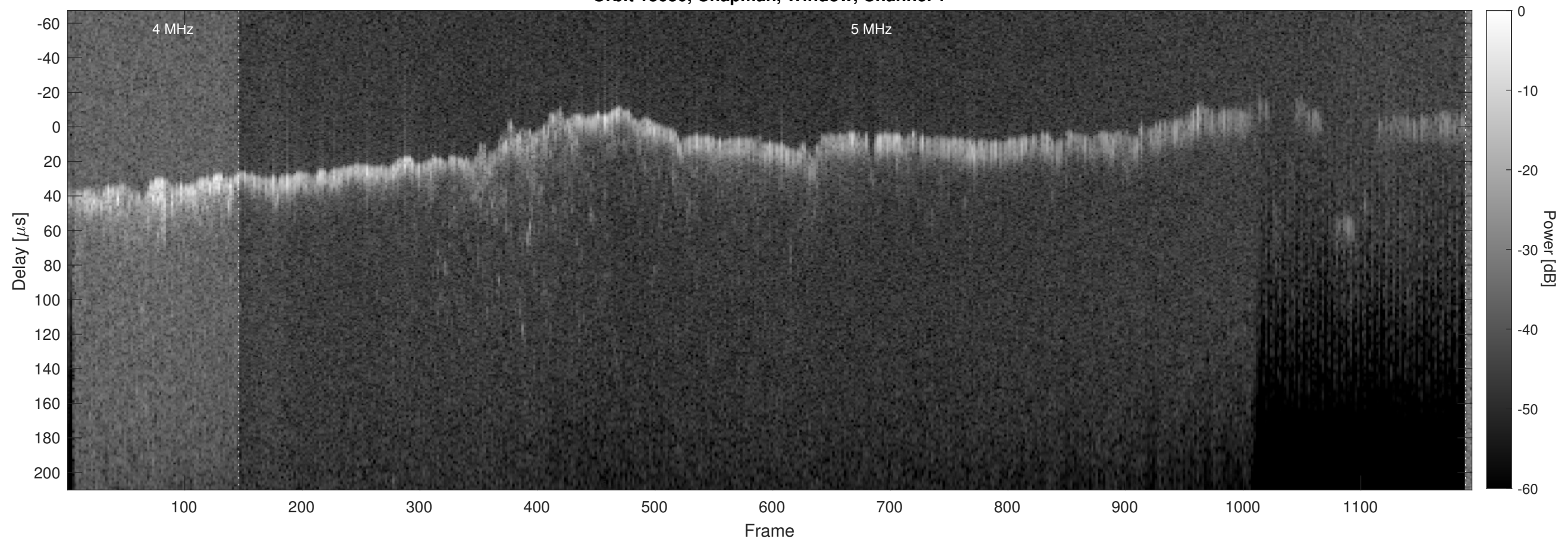
Orbit 13630, Chapman, Window, Channel 2
