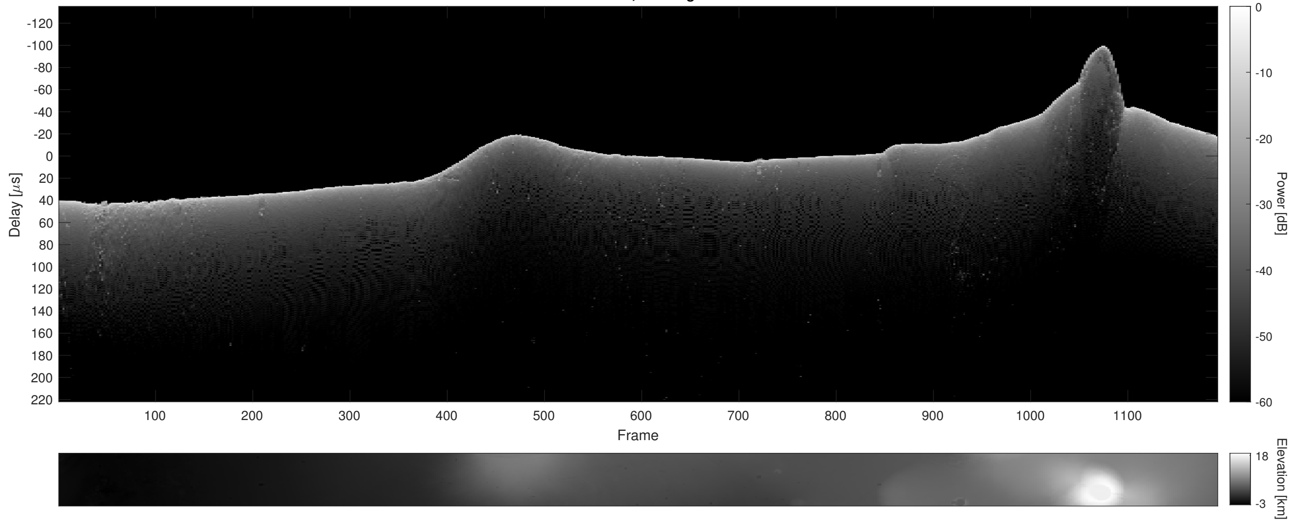
Orbit 13634, Cluttergram
