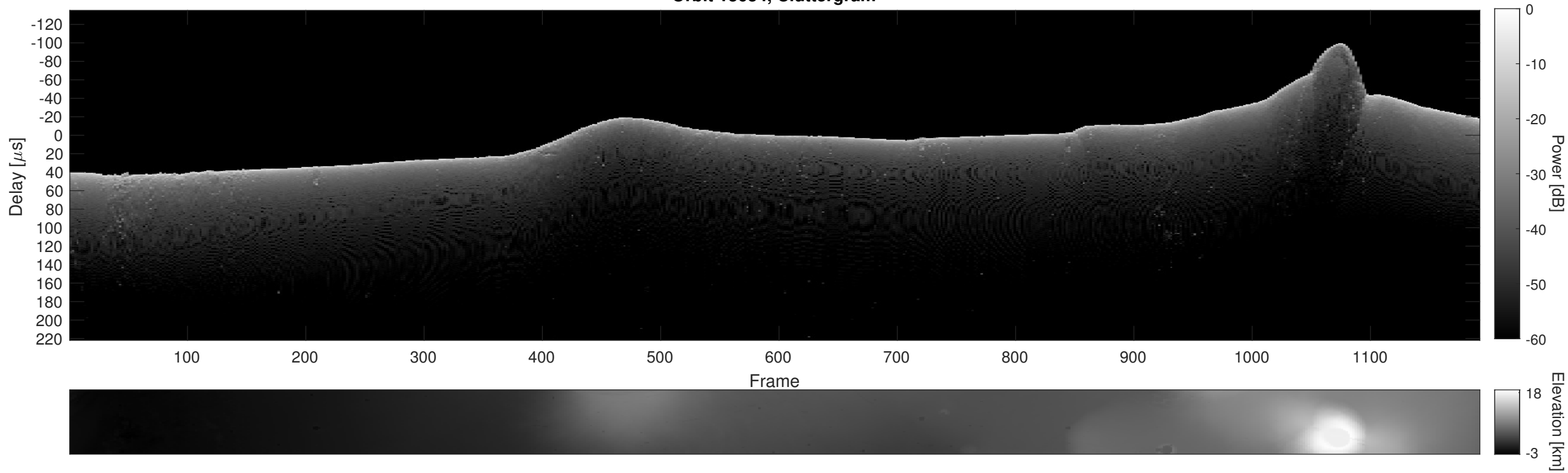
Orbit 13634, Cluttergram
