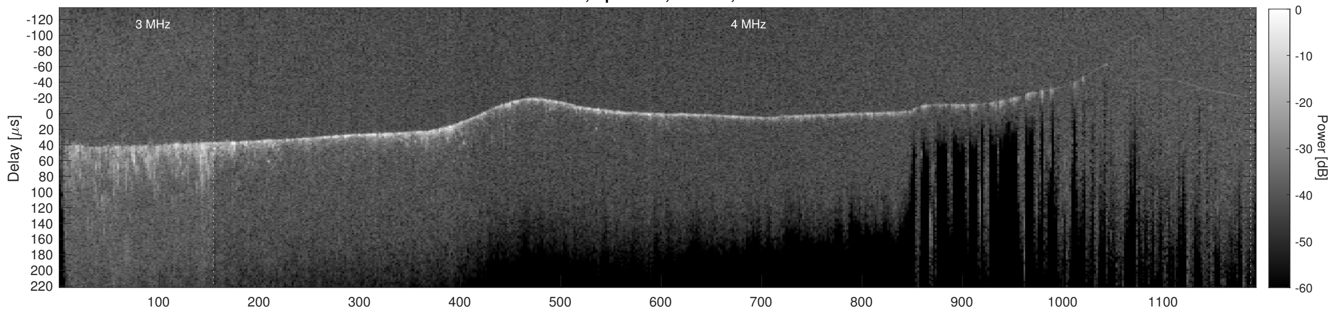
Orbit 13634, Cluttergram
