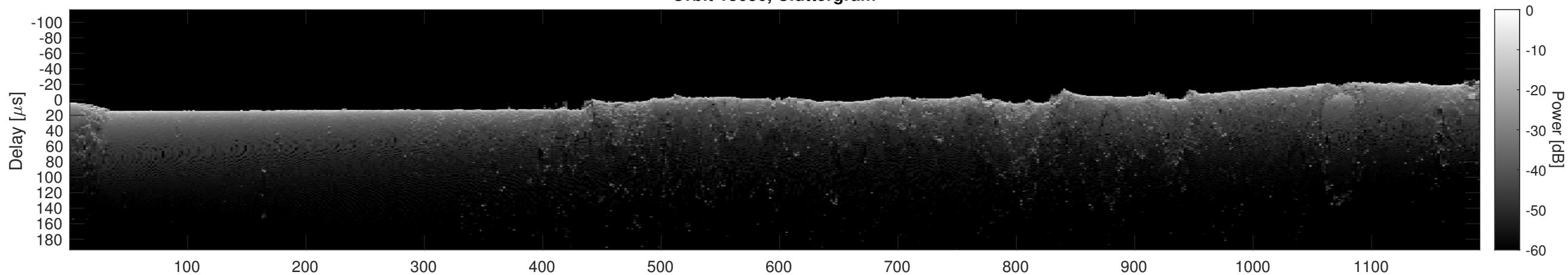
Orbit 13636, Cluttergram
