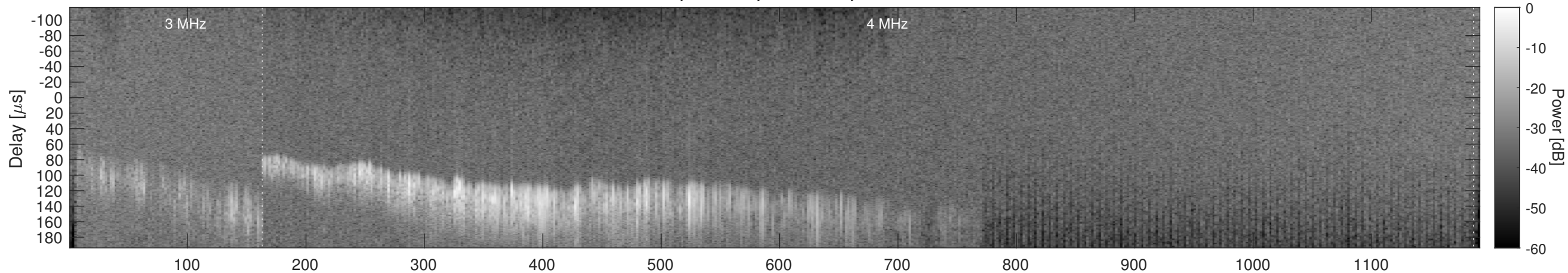
Orbit 13636, Window, Channel 2, Chapman
