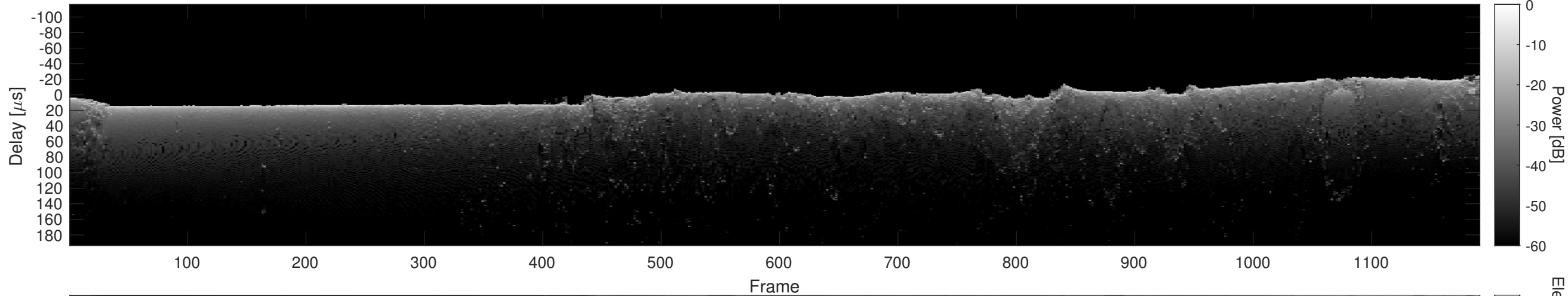
Orbit 13636, Cluttergram
