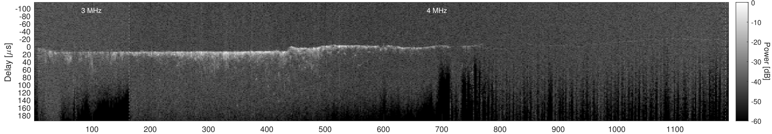
Orbit 13636, Cluttergram
