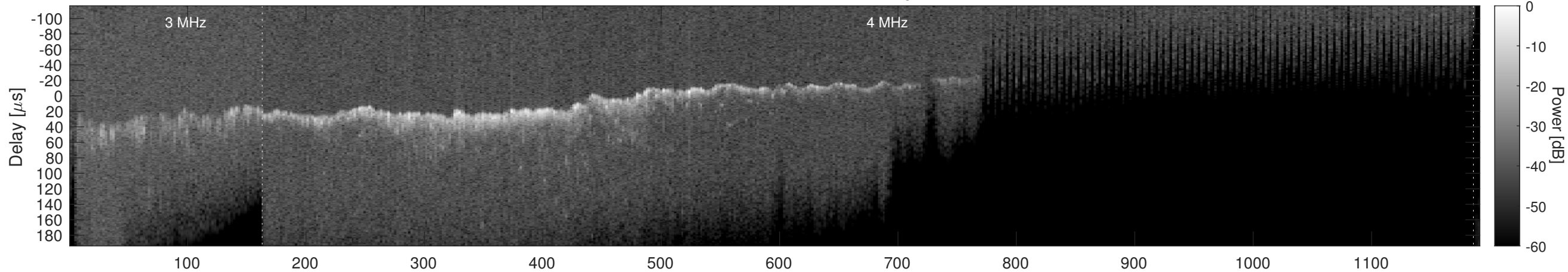
Orbit 13636, Window, Channel 2, Optimized
