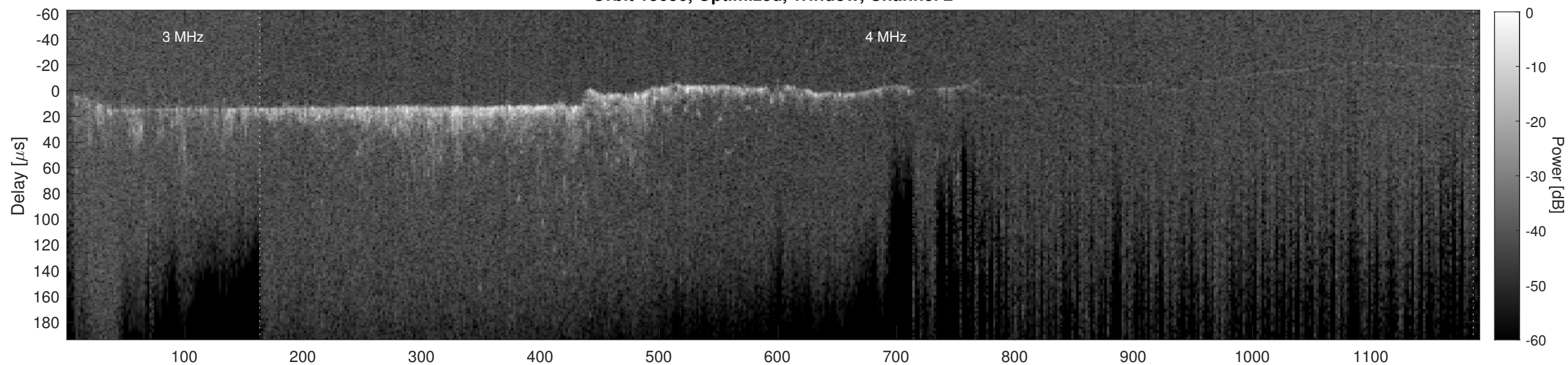
Orbit 13636, Cluttergram
