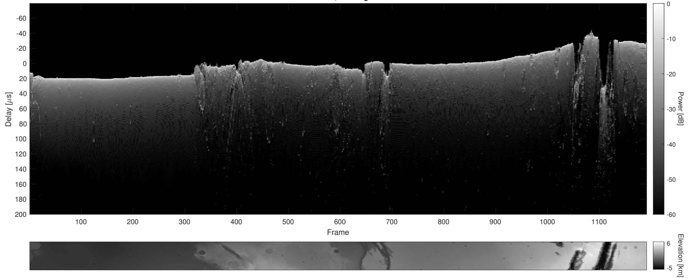
Orbit 13637, Cluttergram
