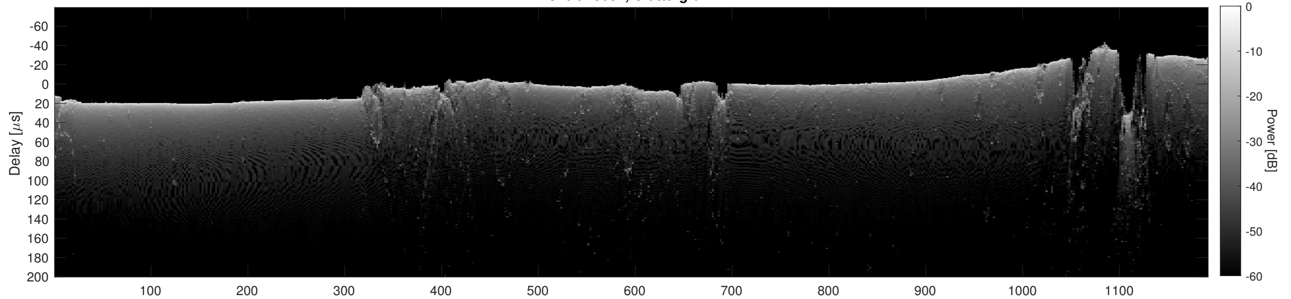
Orbit 13637, Cluttergram
