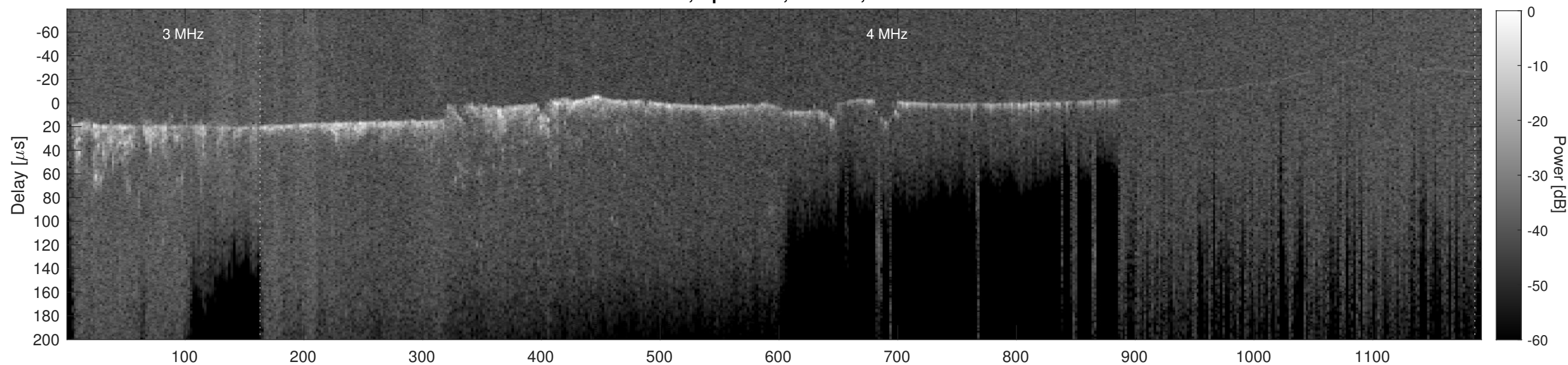
Orbit 13637, Cluttergram
