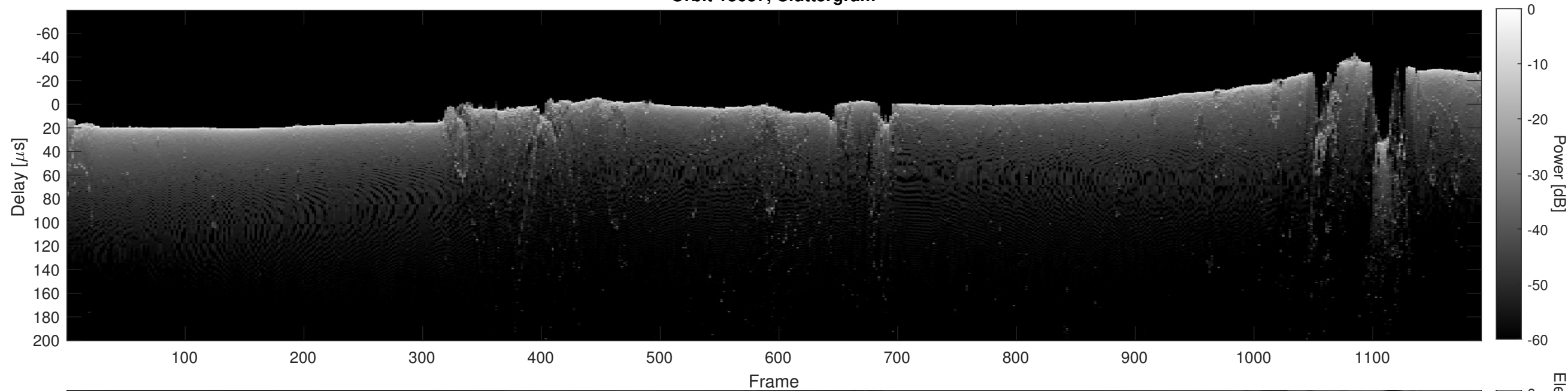
Orbit 13637, Cluttergram
