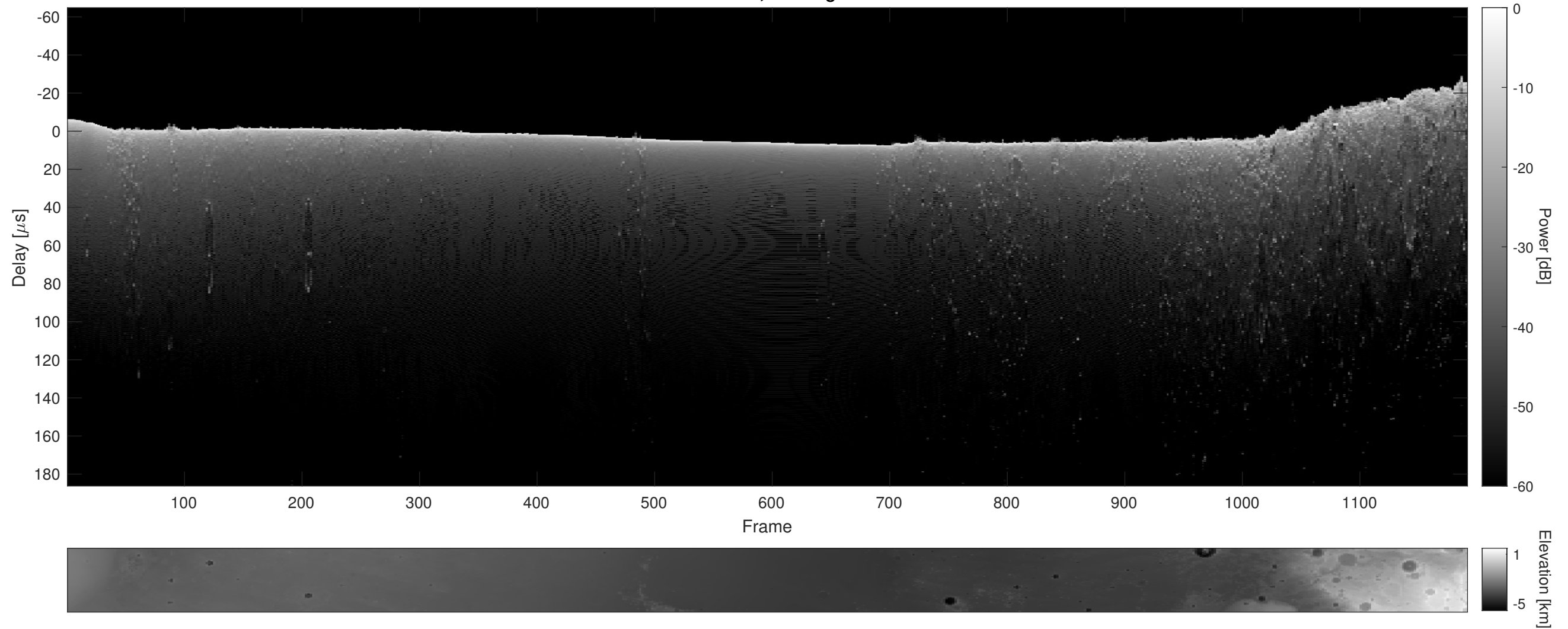
Orbit 13638, Cluttergram
