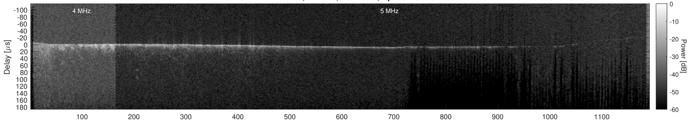
Orbit 13638, Cluttergram
