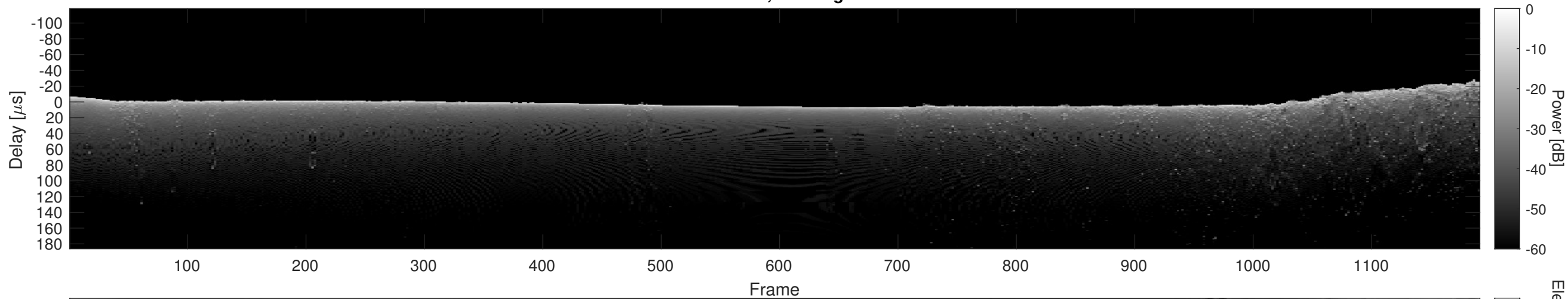
Orbit 13638, Cluttergram
