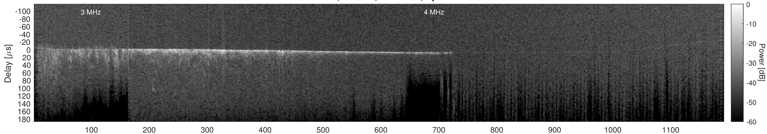
Orbit 13638, Cluttergram
