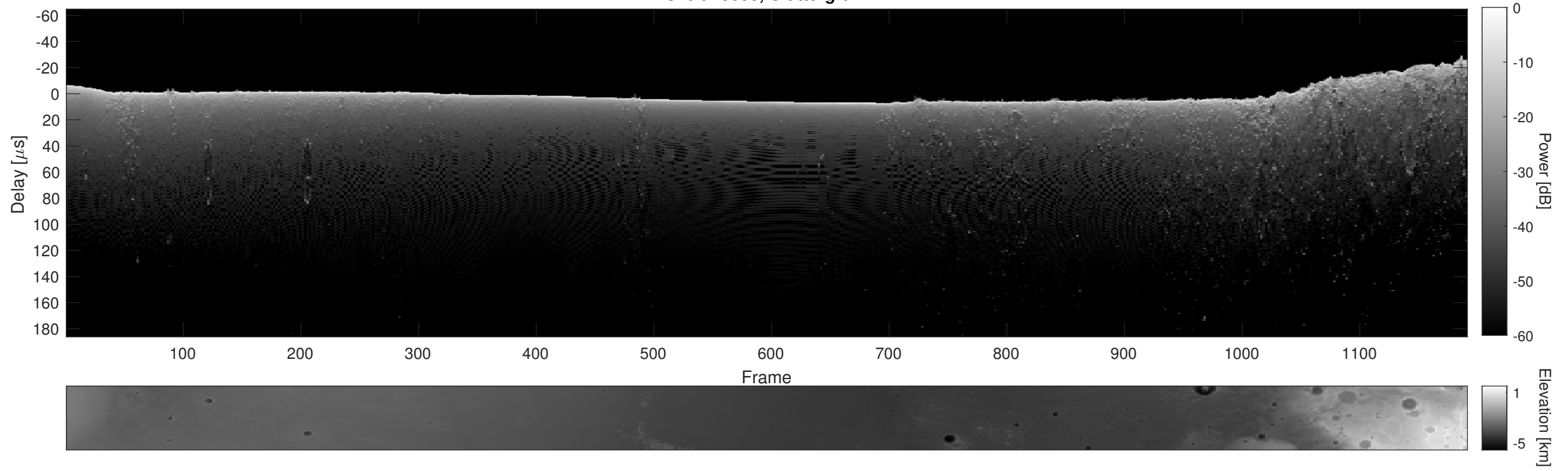
Orbit 13638, Cluttergram
