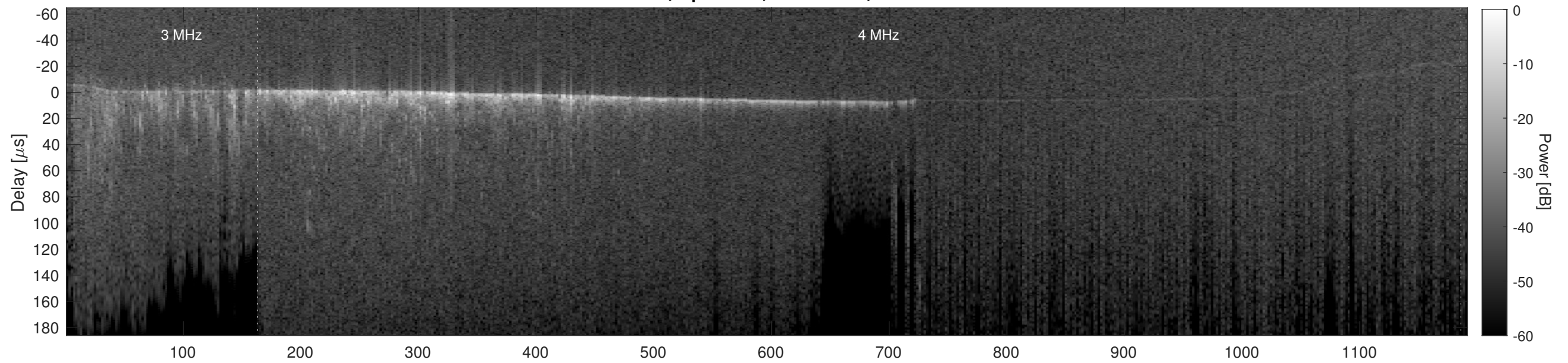
Orbit 13638, Cluttergram
