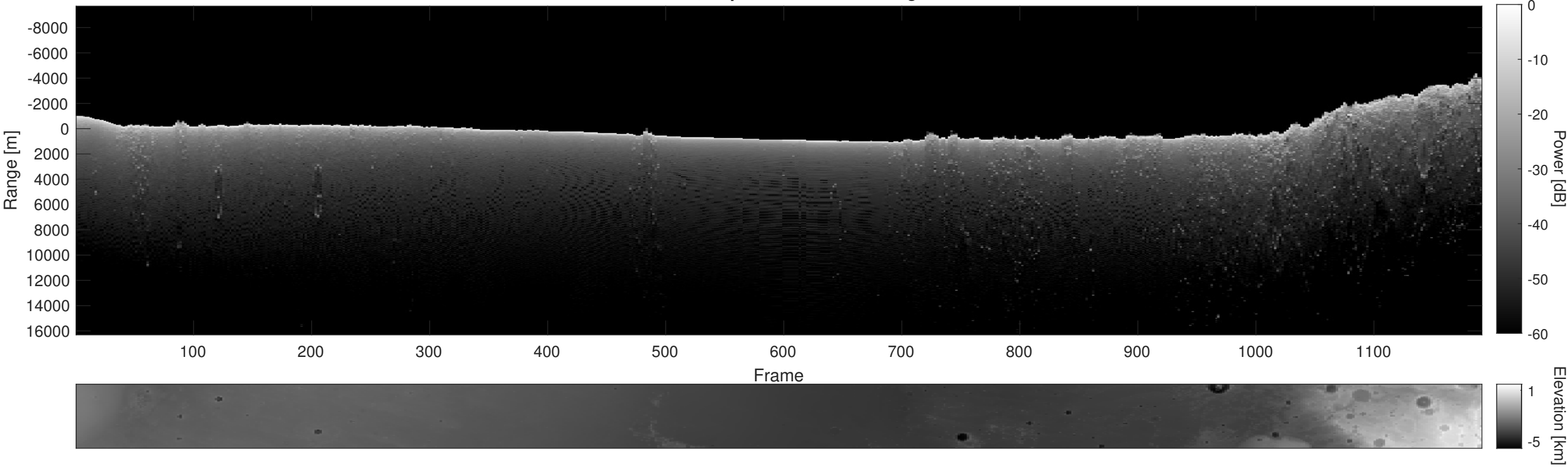
Orbit 13638, Depth-Corrected Cluttergram
