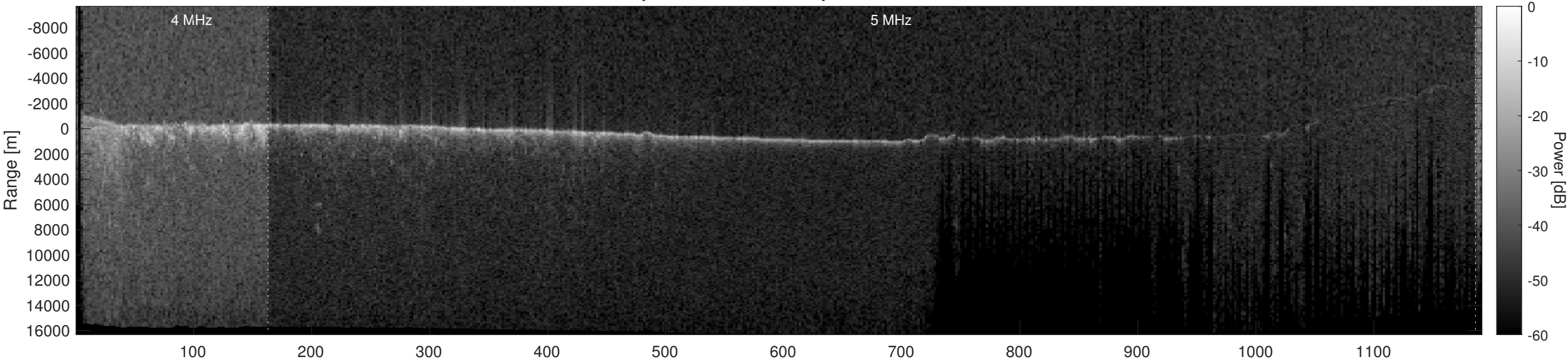
Orbit 13638, Optimized, Window, Depth-Corrected, Channel 2
