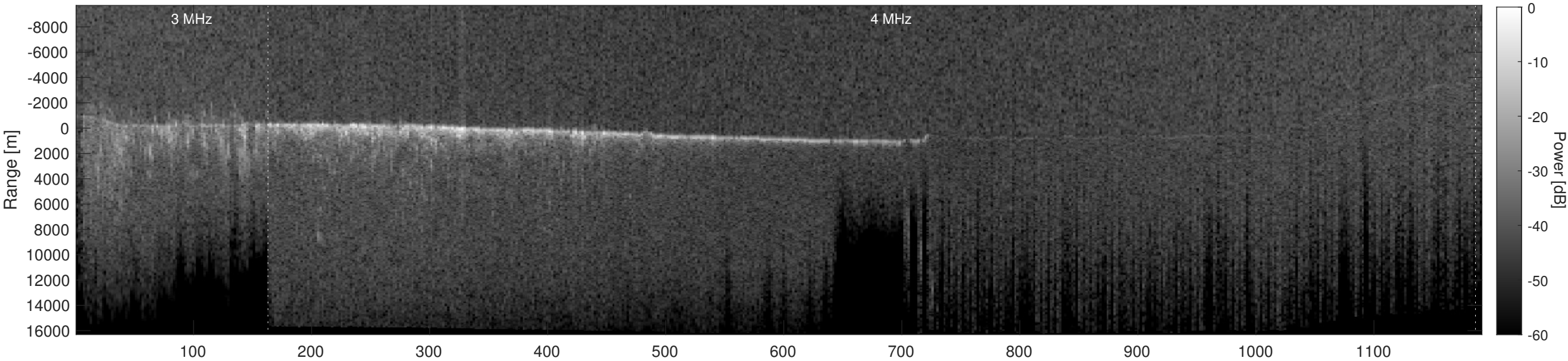
Orbit 13638, Depth-Corrected Cluttergram
